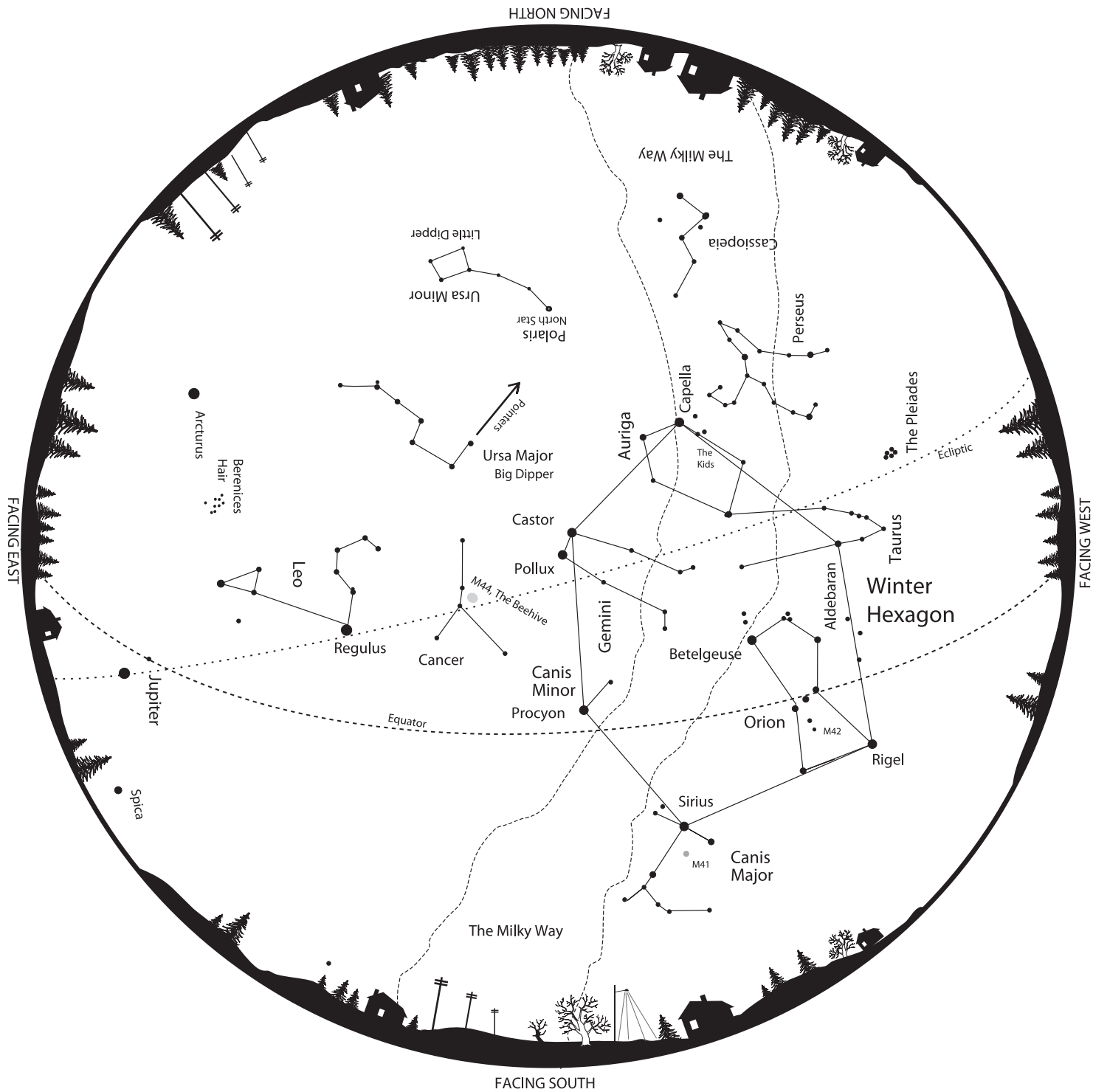
MARCH ALL-SKY CHART EARLY MARCH – 9:30PM LATE MARCH – 8PM
